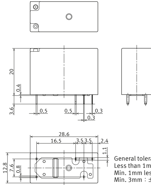
External dimensions
