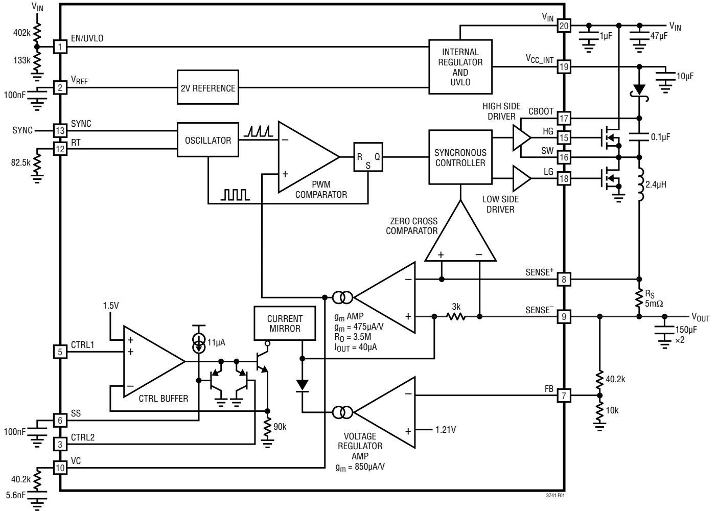
Figure 2. Block Diagram, LT3741-1
