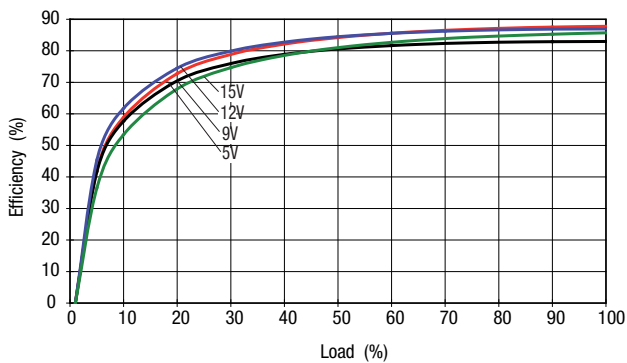
MEV3S05XXSC Input Voltage
