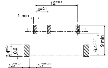
4 mm pitch/ 3-circuit with plugged up hole
