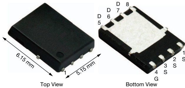
PowerPAK® SO-8 Single
