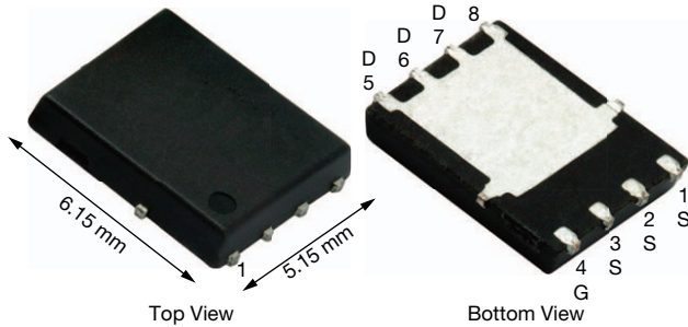
PowerPAK® SO-8 Single
