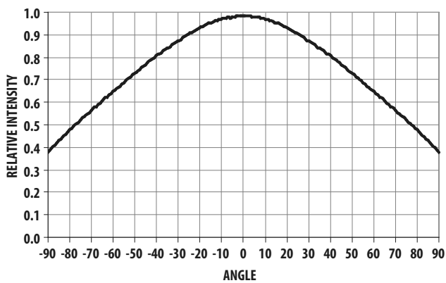
Figure 5: Radiation Pattern
