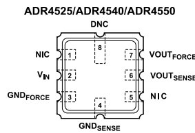
Figure 4. 8-Lead LCC Pin Configuration
