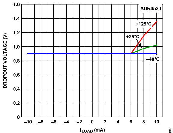
Figure 7. ADR4520 Dropout Voltage vs. Load Current
