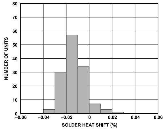
Figure 80. ADR4540 Solder Heat Resistance Shift (3 x Reflow)
