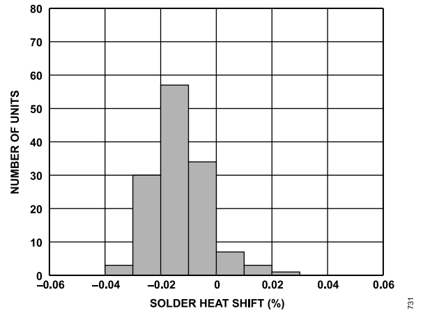
Figure 33. ADR4525 Solder Heat Resistance Shift (3 × Reflow)
