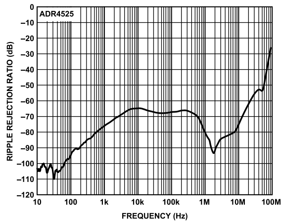
Figure 29. ADR4525 Ripple Rejection Ratio vs. Frequency
