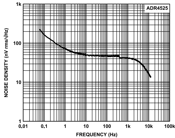
Figure 28. ADR4525 Output Noise Spectral Density
