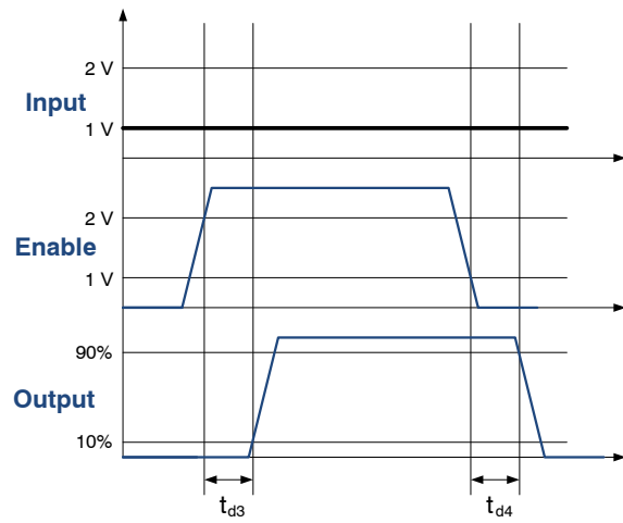
Figure 3. Enable Function for Inverting Input Driver Operation
