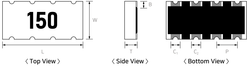
(3) Short-free & Inverted Concave Type
