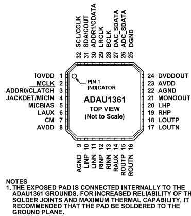
Figure 7. Pin Configuration
