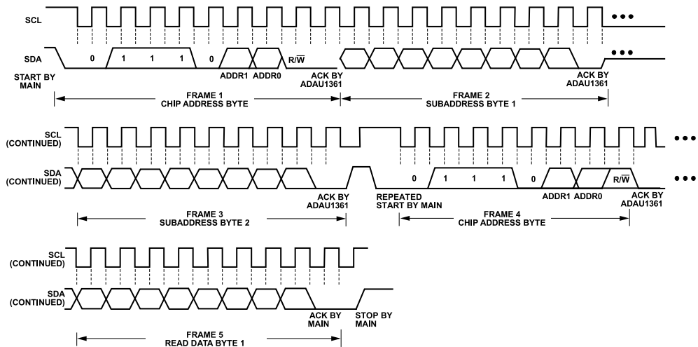
Figure 49. I 2 C Read from ADAU1361 Clocking
