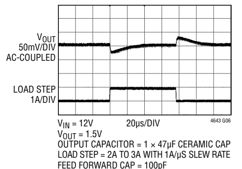
1.5V Output Transient Response
