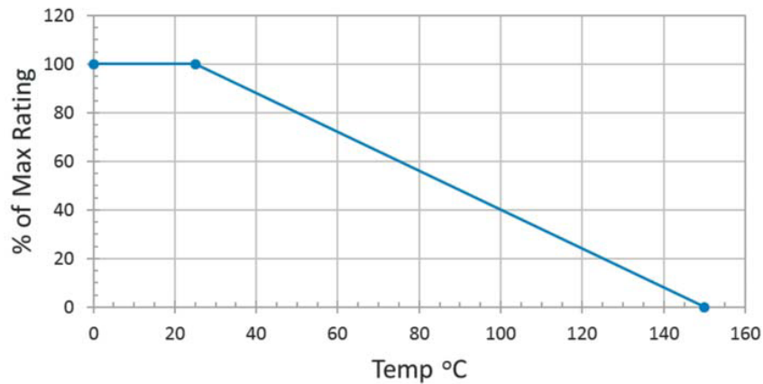
GG Series Temperature Derating Curve
