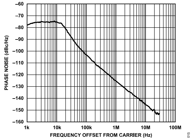
Figure 15. Closed-Loop Phase Noise, RF_{OUTB} = 13.6 GHz, 2x VCO, VCO = 6.8 GHz, f_{PPD} = 61.44 MHz, Loop Bandwidth = 10 kHz
