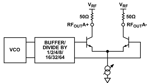
Figure 34. Output Stage
