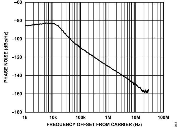
Figure 13. Closed-Loop Phase Noise, RF_{OUTB} = 6.8 GHz, 2x VCO, VCO = 3.4 GHz, f_{PPD} = 61.44 MHz, Loop Bandwidth = 10 kHz
