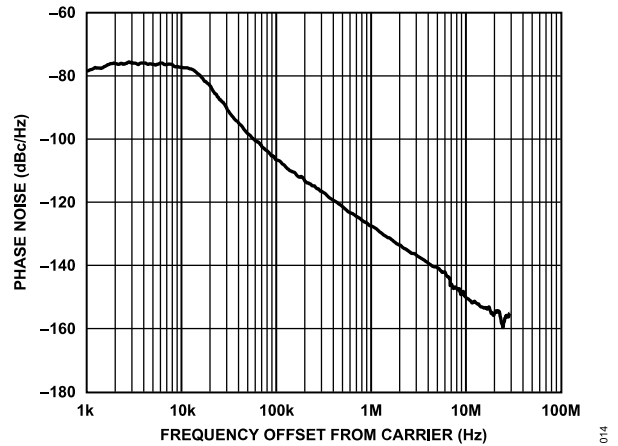
Figure 14. Closed-Loop Phase Noise, RF_{OUTB} = 10 GHz, 2x VCO, VCO = 5.0 GHz, f_{PPD} = 61.44 MHz, Loop Bandwidth = 10 kHz
