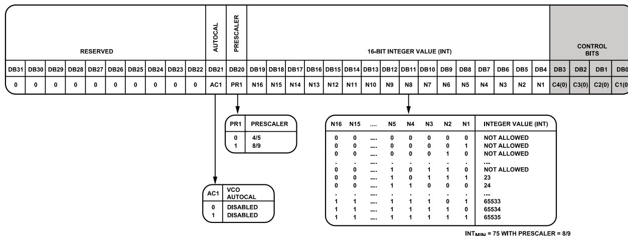
Figure 38. Register 0 Details
