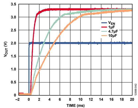
Figure 40. V_{OUT} Start-Up Time Behavior at Various Values of C_{BY} , V_{OUT} = 3.3 \text{ V}
