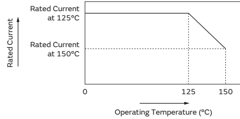
Derating of Rated Current
