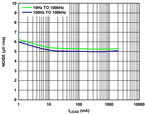
Figure 41. RMS Output Noise vs. Load Current ( I_{LOAD} ), V_{OUT} = 5 V
