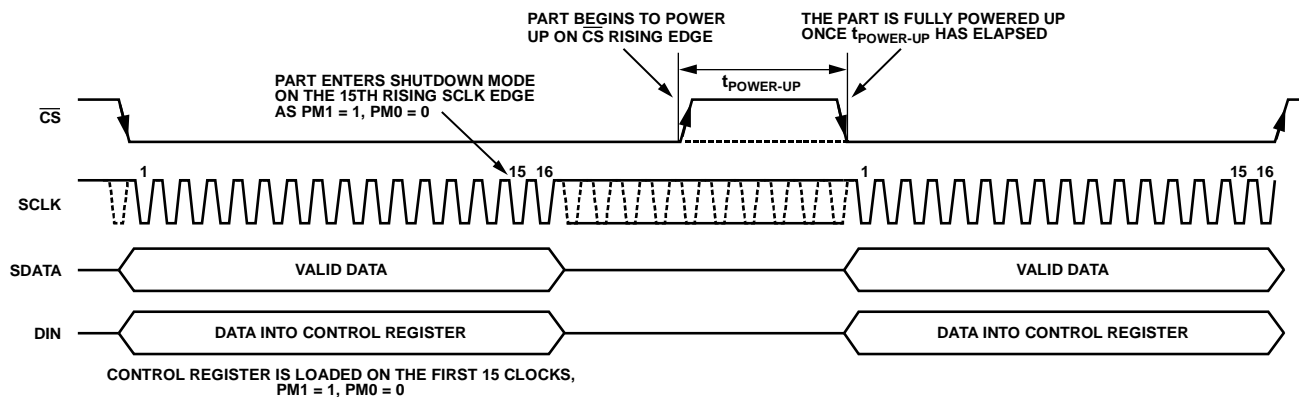
Figure 50. Entering Autos shutdown/Autostandby Mode
