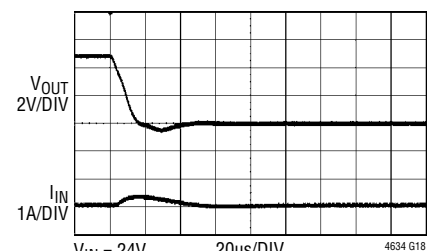
24V to 5V No Load Short
