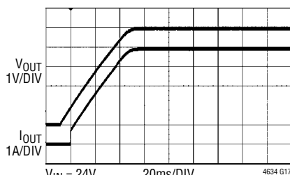
24V to 5V Full Load Start-Up
