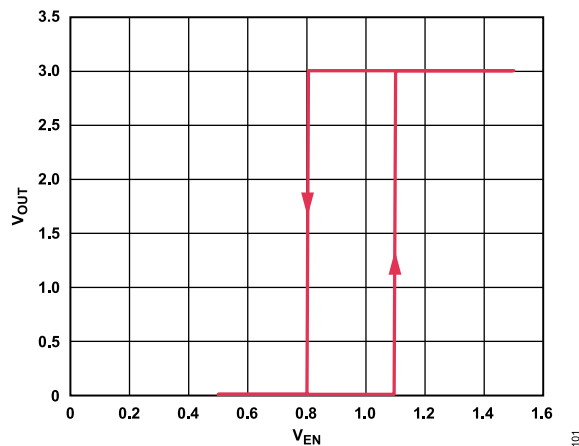
Figure 30. Typical EN Pin Operation
