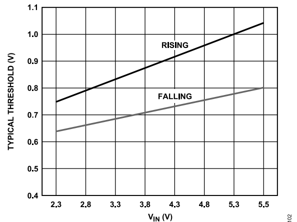
Figure 31. Typical EN Pin Thresholds vs. Input Voltage (V IN )
