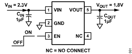
Figure 1. 5-Lead TSOT with Fixed Output Voltage, 1.8 V
