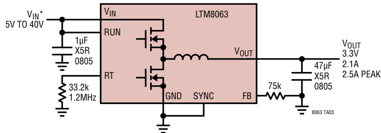
3.3V OUT from 5V IN to 40V IN Step-Down Converter
