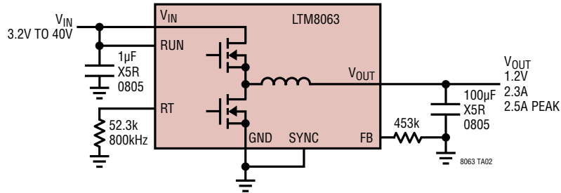
1.2V OUT from 3.2V IN to 40V IN Step-Down Converter
