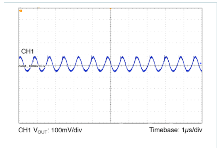
Figure 38 — Output ripple 24VIN, 15.0V OUT at 8A
