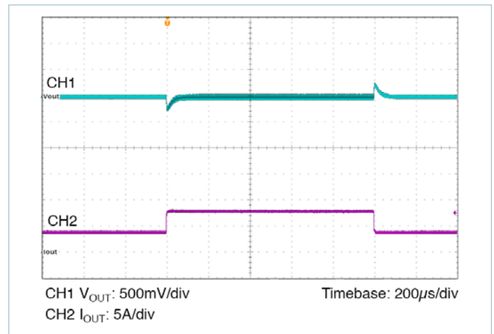
Figure 28 — Transient response 4A to 8A, at 5A/µs
