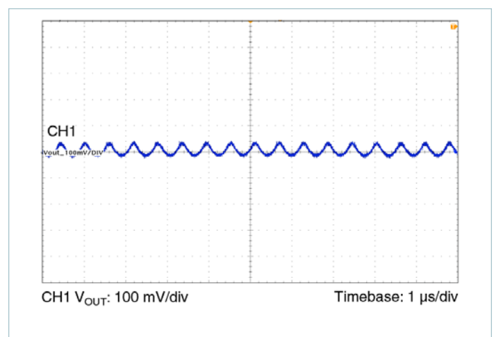
Figure 39 — Output ripple 24VIN, 15.0V OUT at 4A
