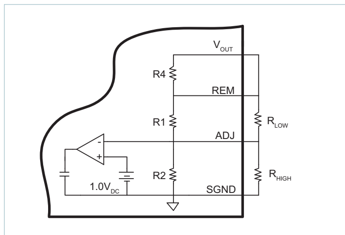
Figure 45 — Internal resistor divider network
