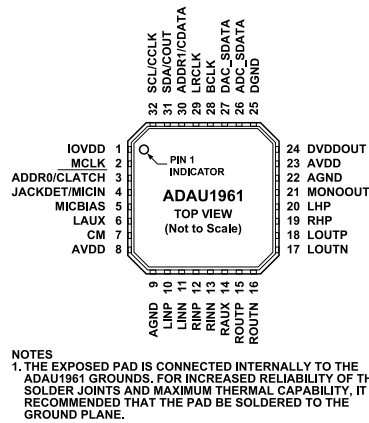
Figure 7. Pin Configuration
