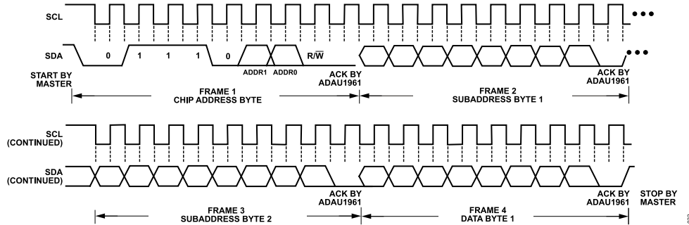
Figure 48. I 2 C Write to ADAU1961 Clcking
