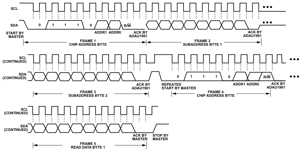
Figure 49. I 2 C Read from ADAU1961 Clcking
