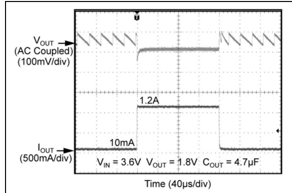
FIGURE 2-28: Load Transient (10 mA to 1.2A).
