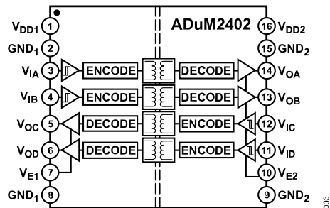
Figure 3. ADuM2402
