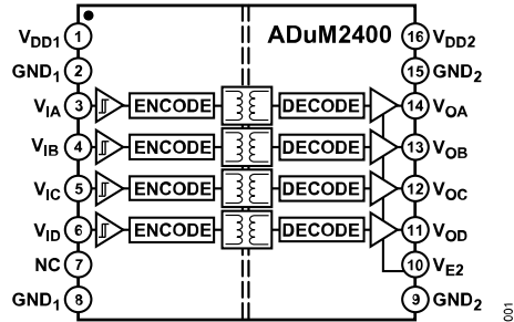
Figure 1. ADuM2400
