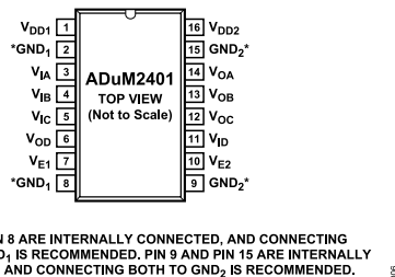
Figure 6. ADuM2401 Pin Configuration
