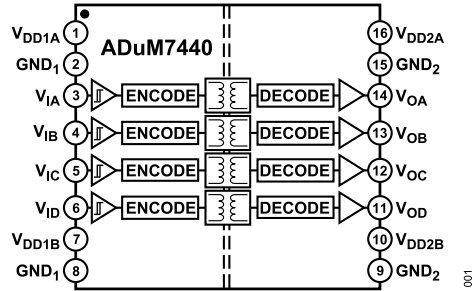
Figure 1. ADuM7440
