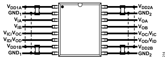
Figure 16. Recommended Printed Circuit Board Layout
