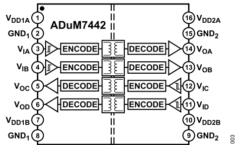
Figure 3. ADuM7442
