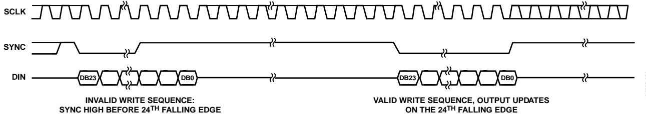
Figure 40. SYNC Interrupt Facility
