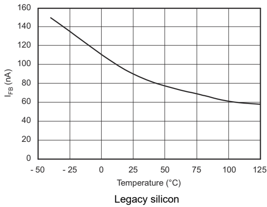
Figure 5-49. TPS73601 I_{FB} vs Temperature
