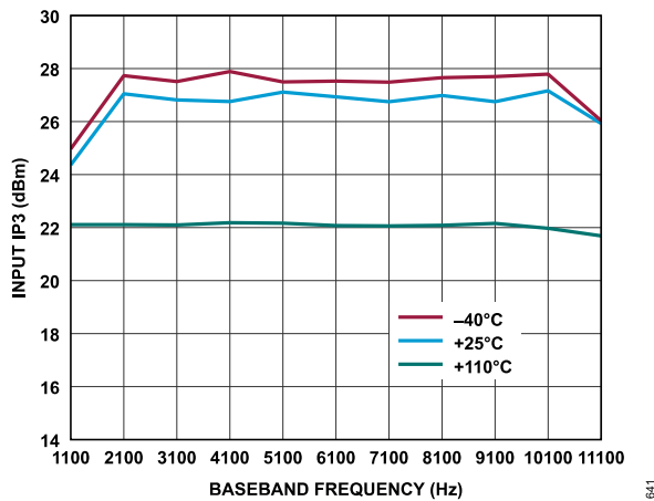
Figure 330. Receiver Input IP3 vs. Baseband Frequency, ADC = High Performance, f_1 = \text{Baseband Frequency} + 1 \text{ MHz} , f_2 = \text{Baseband Frequency} + 2 \text{ MHz} , Gain Index = 255, First-Order TIA with f_{1dB} = 4 \text{ MHz} , P_{OUT} = -12.6 \text{ dBFS} at -40^\circ\text{C} and +25^\circ\text{C} , P_{OUT} = -15.6 \text{ dBFS} at +110^\circ\text{C}
