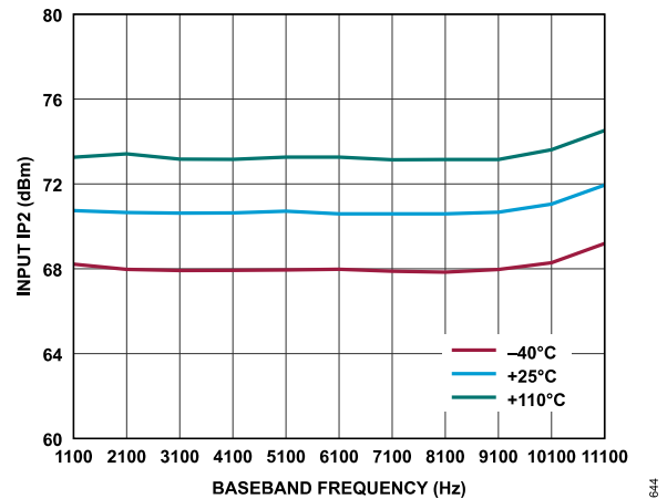
Figure 323. Receiver Input IP2 vs. Baseband Frequency, ADC = Low Power, f_1 = \text{Baseband Frequency} + 1 \text{ MHz} , f_2 = \text{Baseband Frequency} + 2 \text{ MHz} , Gain Index = 255, First-Order TIA with f_{3dB} = 4 \text{ MHz} , P_{OUT} = -6.6 \text{ dBFS}
