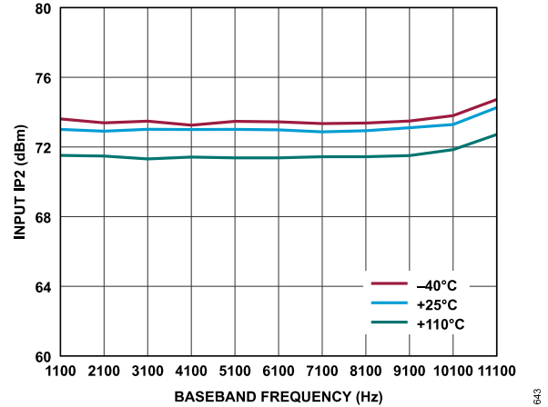
Figure 322. Receiver Input IP2 vs. Baseband Frequency, ADC = High Performance, f_1 = \text{Baseband Frequency} + 1 \text{ MHz} , f_2 = \text{Baseband Frequency} + 2 \text{ MHz} , Gain Index = 255, First-Order TIA with f_{3dB} = 4 \text{ MHz} , P_{OUT} = -6.6 \text{ dBFS}
