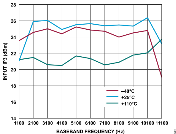
Figure 331. Receiver Input IP3 vs. Baseband Frequency, ADC = Low Power, f_1 = \text{Baseband Frequency} + 1 \text{ MHz} , f_2 = \text{Baseband Frequency} + 2 \text{ MHz} , Gain Index = 255, First-Order TIA with f_{1dB} = 4 \text{ MHz} , P_{OUT} = -12.6 \text{ dBFS} at -40^\circ\text{C} and +25^\circ\text{C} , P_{OUT} = -15.6 \text{ dBFS} at +110^\circ\text{C}
